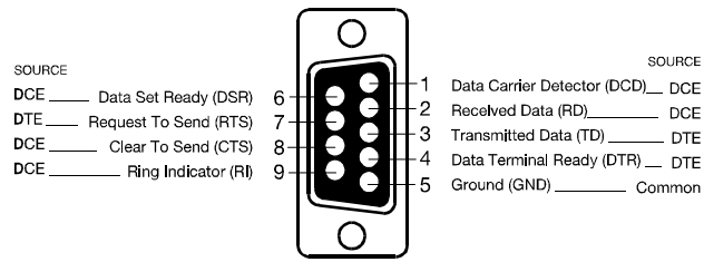
PC D-sub 9 Standard Connection
