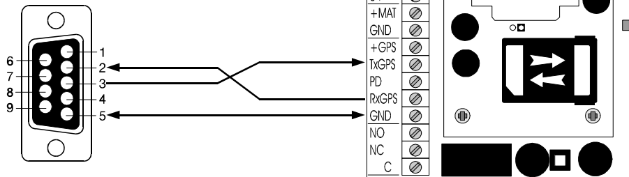
D-sub 9 pole Female
